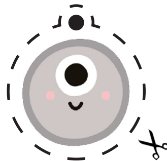
Mercuri
